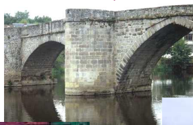
1205 Pont St Martial Limoges France
