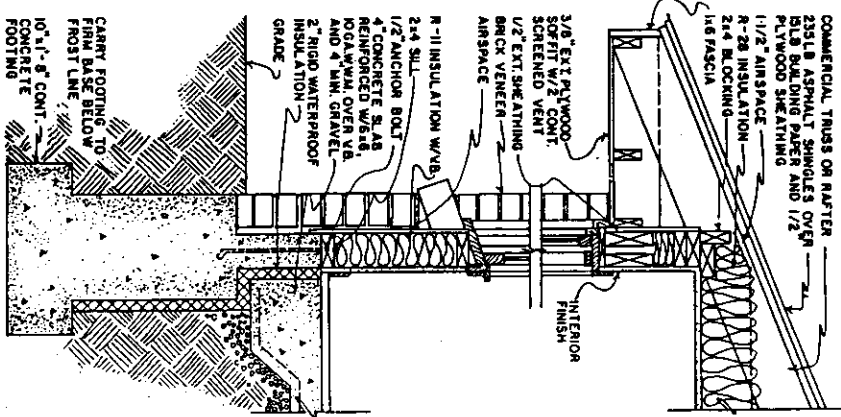
BRICK VENEER SLAB ON GRADE SHOWN W/WOOD DOUBLE HUNG WINDOWS
