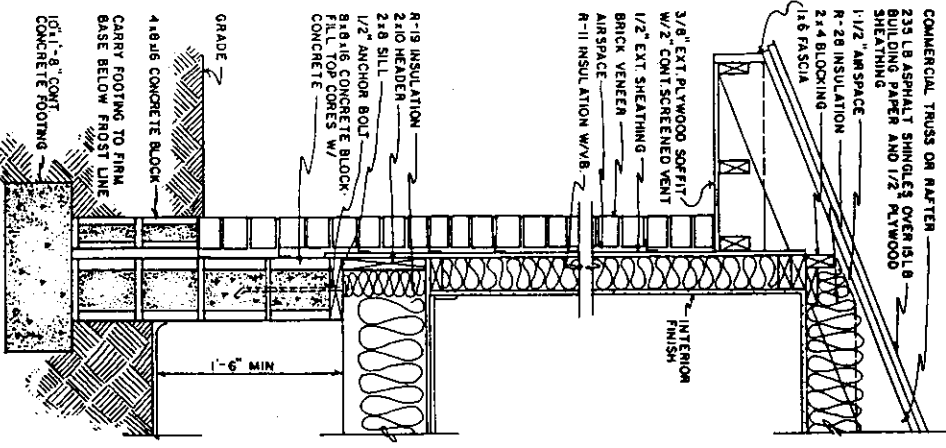
BRICK VENEER W/CRAWL SPACE OR BASEMENT
