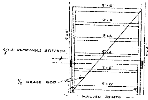
DOOR FRAMING SCALE 1/2" = 1'-0"
