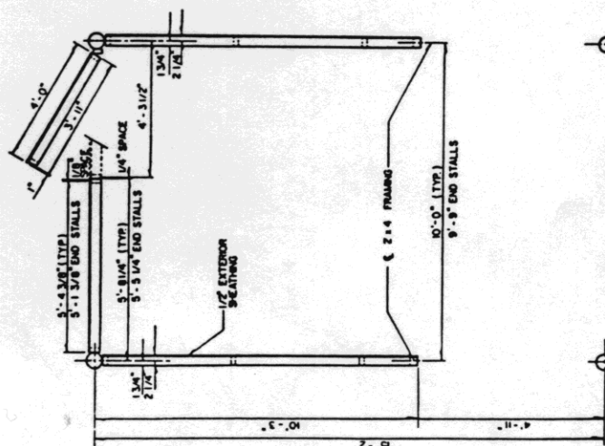
STALL PLAN
