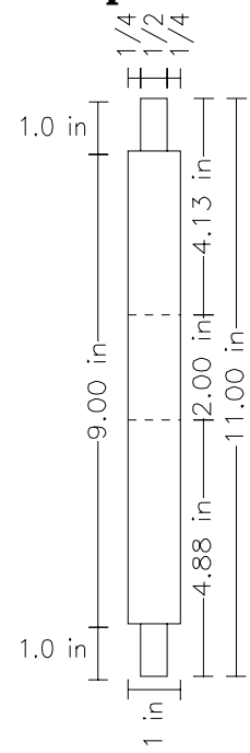
Top View
