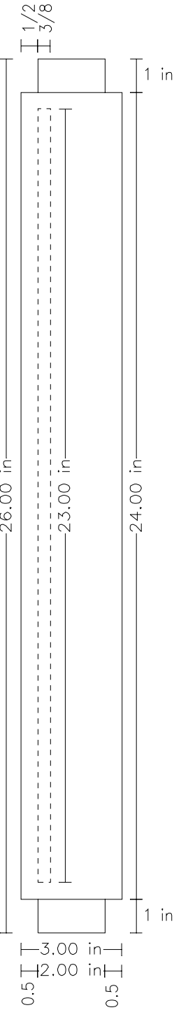
Front View
