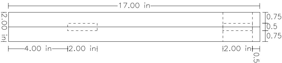
Side View
