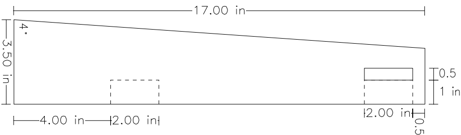
Top View
