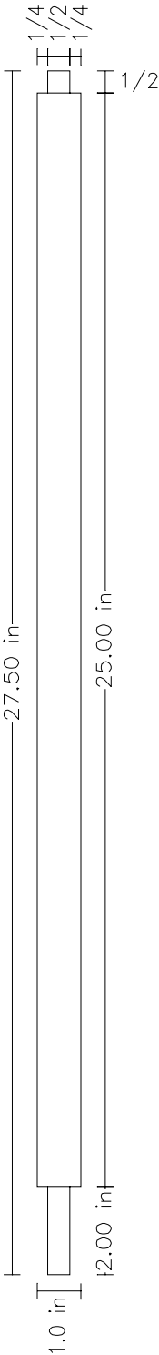
Front View
