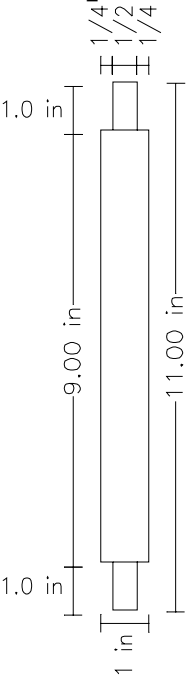
Top View
