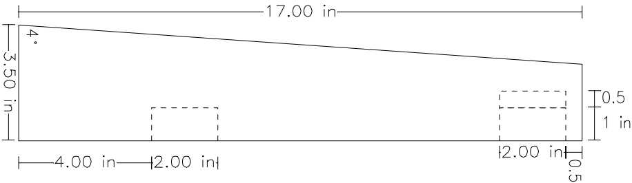
Side View
