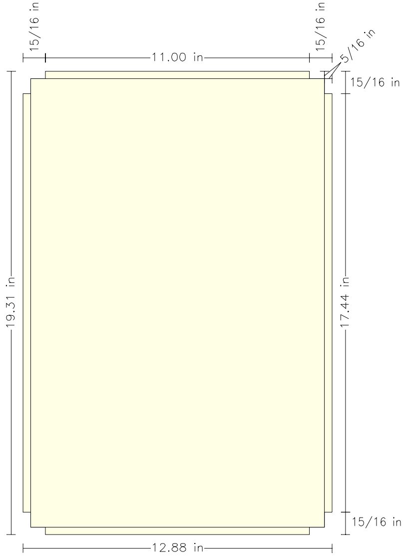
Top View
