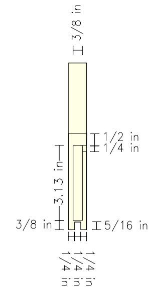
Rear View
