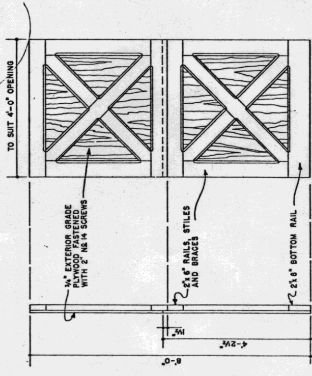
USE HEAVY DUTY HINGES AND DOOR BOLTS
