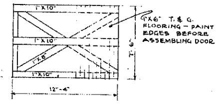
SLIDING DOOR SCALE \frac{3}{16}'' = 1'-0''
