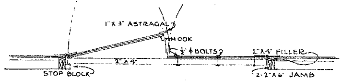
BAR FOR BOTTOM OF HINGED DOORS SCALE \frac{3}{8}'' = 1'-0''
