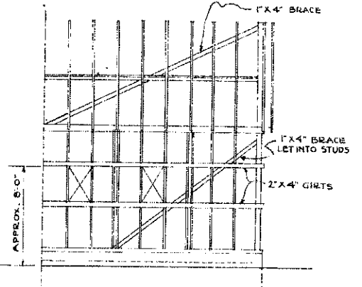
FRAMING DIAGRAM OF REAR WALL SCALE \frac{1}{8}'' = 1'-0''
