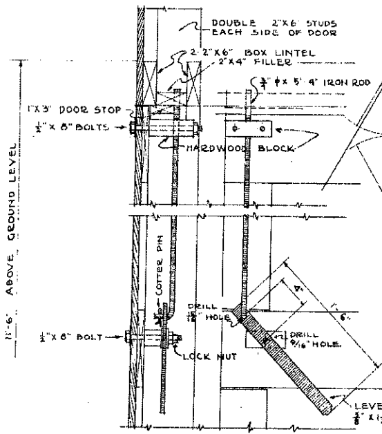
SECTION INSIDE ELEVATION DETAIL OF LOCKING DEVICE FOR SWINGING DOOR SCALE 1\frac{1}{2}'' = 1'-0''
