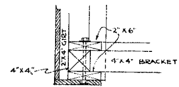
DETAIL CORNER POST (SECT B-B) SCALE 1\frac{1}{2}'' = 1'-0''
