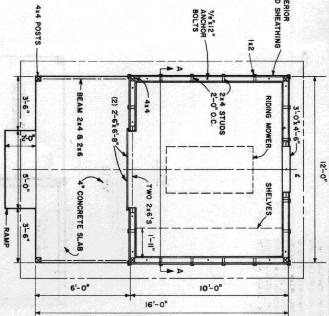
PLAN SCALE: 0 1 2 3 4 FT.
