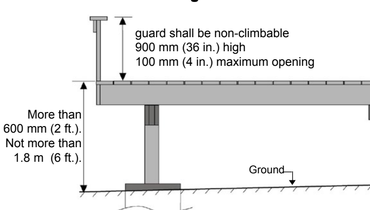
FIGURE 11 - Guardrail Height
