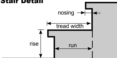
FIGURE 14 - Stair Detail
