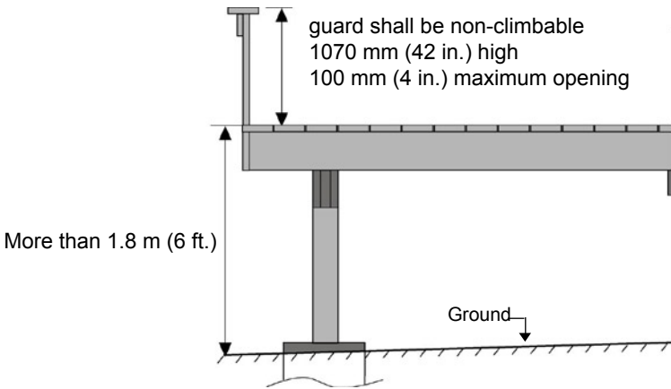
FIGURE 12 - Guardrail Height
