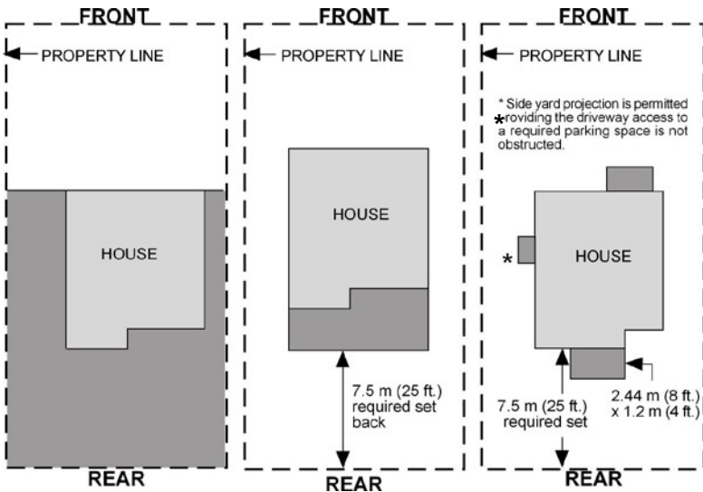
FIGURE 4 - Deck Location
