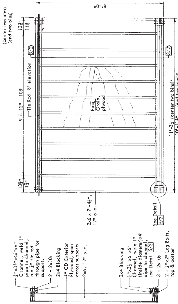
BULKHEAD CROSS SECTION—3/2
