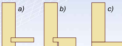
Drawer bottom possibilities. a) inset 1/4" plywood b) rabbeted 1/2" plywood c) flush trimmed 1/4" plywood
