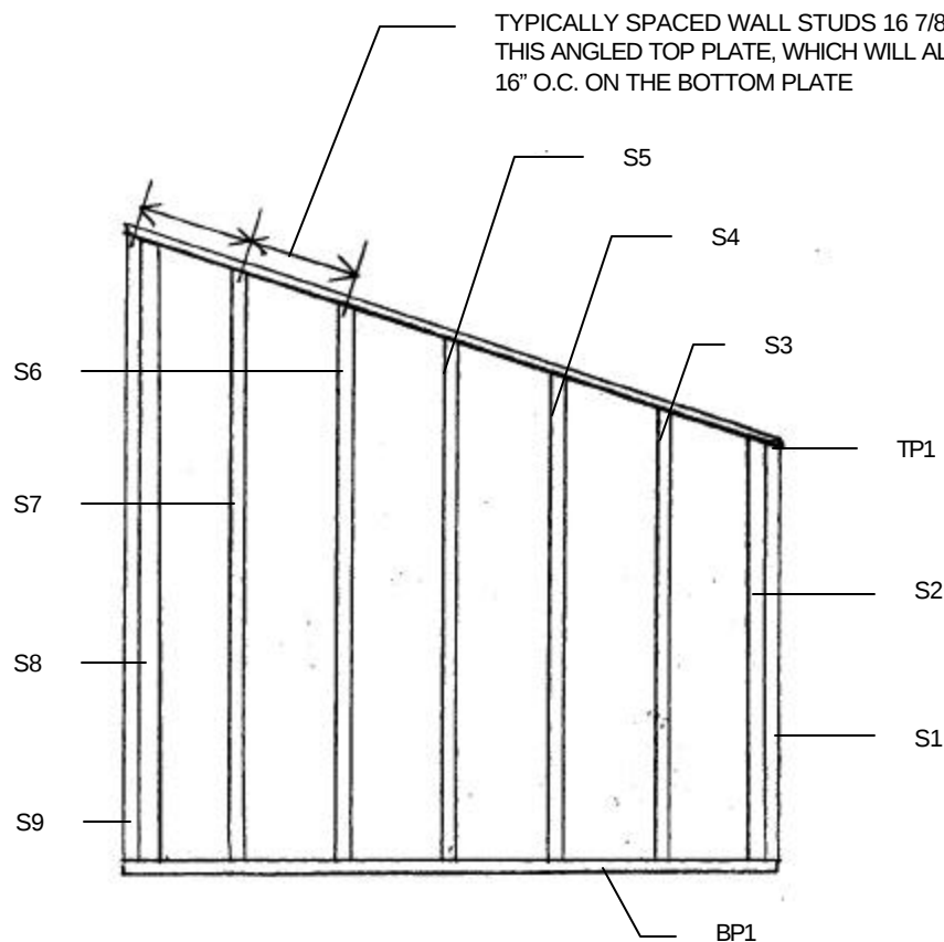
WALL BUILDING STEP # 2
