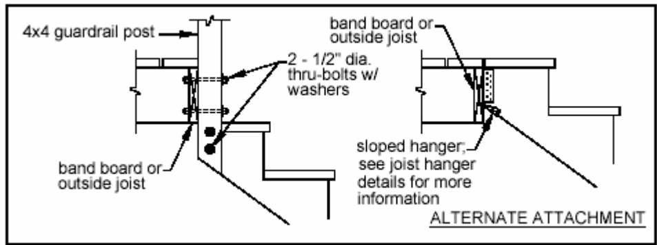
Figure 32 – Stair Stringer Connection Detail
