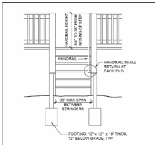
Figure 34 – Misc Stair Requirements
