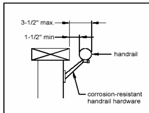
Figure 33 – Handrail Requirements
