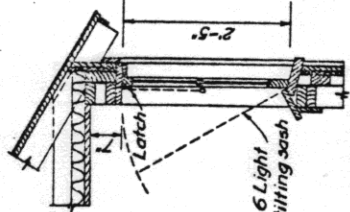
WINDOW DETAIL
