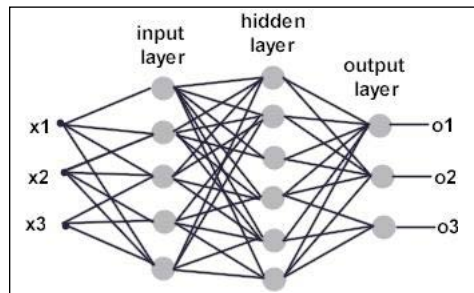
Figure 1.3: A simplified example of a three-layer ANN (input, hidden, output). Input vectors are three-dimensional ([x_1, x_2, x_3]) . All inputs are 'fed' to all input layer nodes. All nodes of a layer are connected to all nodes of the next layer. Weights at connections are not shown for simplicity.
