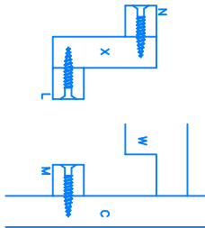
GLIDE DETAIL FIGURE 7
