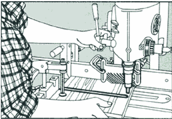
Figure 2 Use the Belt Sander to sand the drawers to fit.
