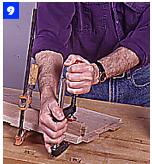
Join the bottom front rail to the case bottom with joining plates and glue. Clamp together until the glue sets.
