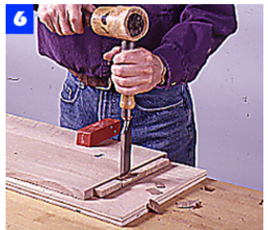
Use a chisel to remove waste between the through tenons. Work from both sides of the board to prevent tearout.
