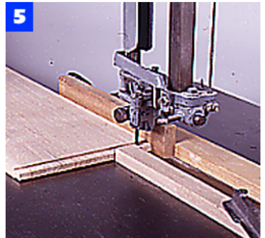
Use a band saw and stopblock to make the shoulder cuts on the through tenons for the top and bottom panels.
