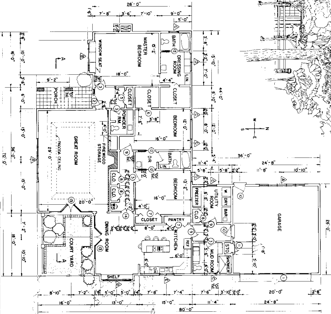
FLOOR PLAN Vol. 4 Kings Highway
