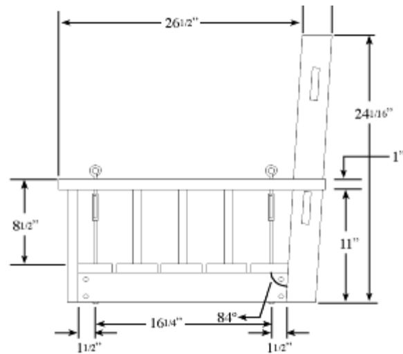
Seat Frame
