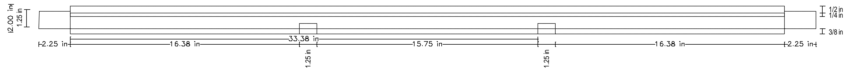
Front View
