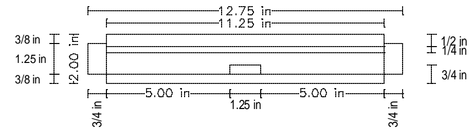
Side View
