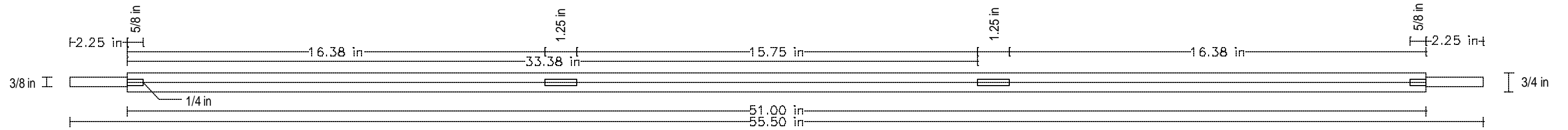
Top View
