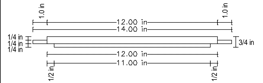
Side View
