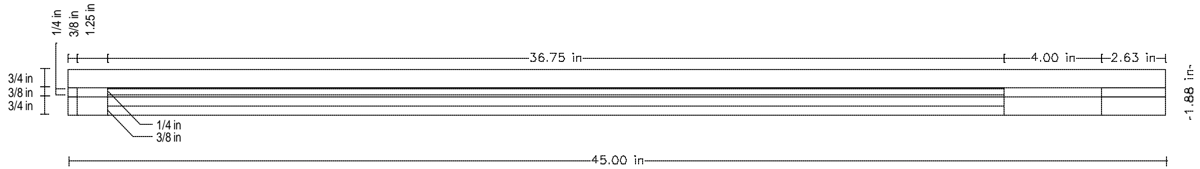
Side View
