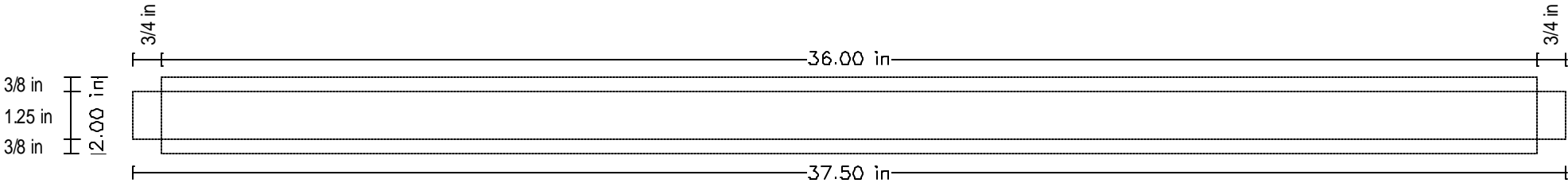
Front View
