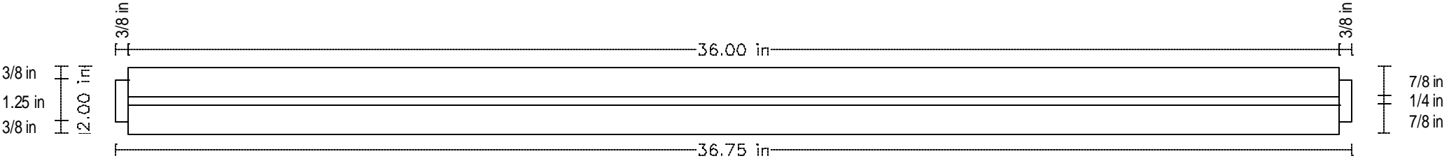
Front View
