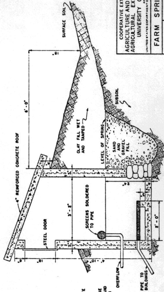
CROSS SECTION ON LINE A-A
