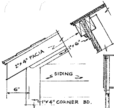
DETAIL OF CORNICE SCALE 1/2" = 1'-0"
