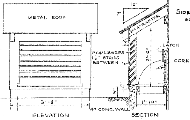
DETAIL OF AIR INTAKE SCALE 3/4" = 1'-0"
