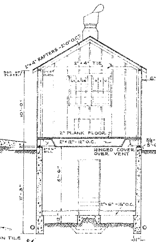
TRANSVERSE SECTION SCALE 1/4" = 1'-0"
