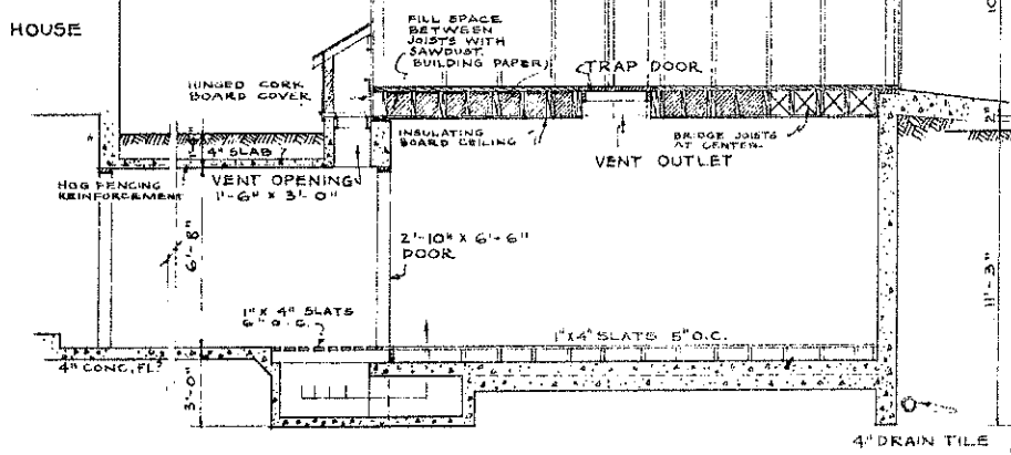
LONGITUDINAL SECTION SCALE 1/4" = 1'-0"
