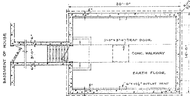
STORAGE ROOM PLAN SCALE 1/4" = 1'-0"
