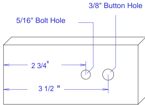
Clamp Jaw Layout (Side 1)
