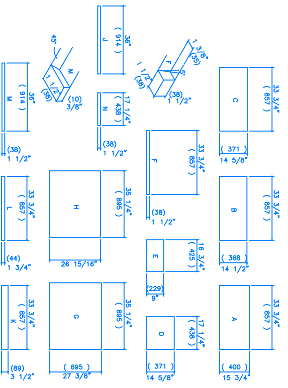
MATERIAL LAYOUT
