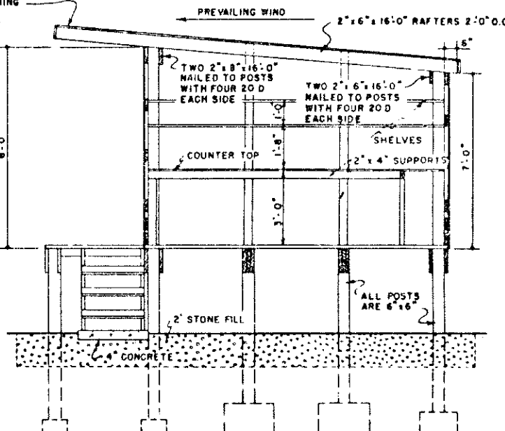
SECTION X-X
