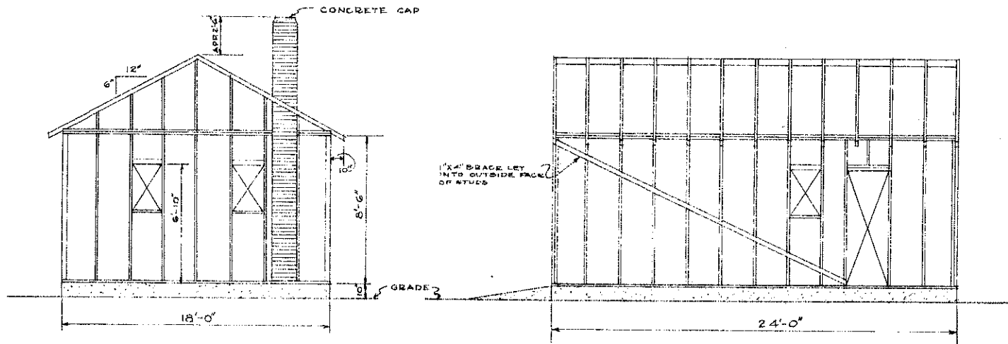
REAR WALL FRAMING SCALE \frac{1}{4}'' = 1'-0''
