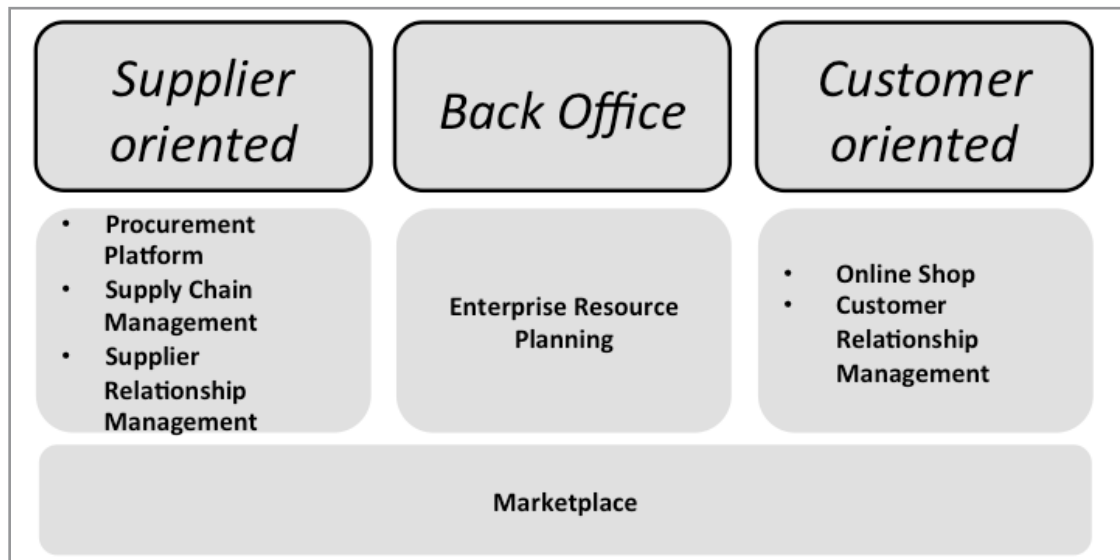
Figure 5: Software architecture
