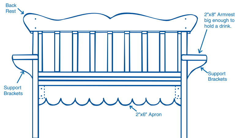
FRONT ELEVATION
