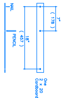
TRAMMEL FIGURE 5
