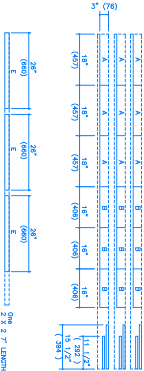
CUTTING DIAGRAM FIGURE 1
