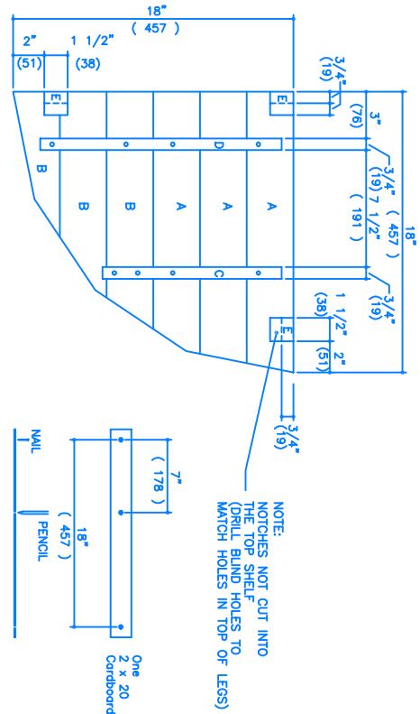
SHELF DETAIL FIGURE 3
