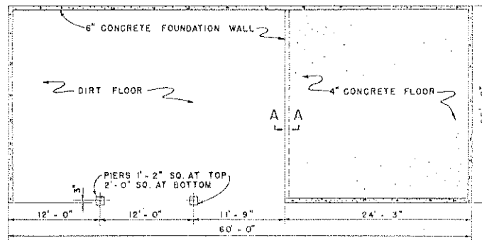
FOUNDATION PLAN SCALE — 1/2" = 1'-0"
