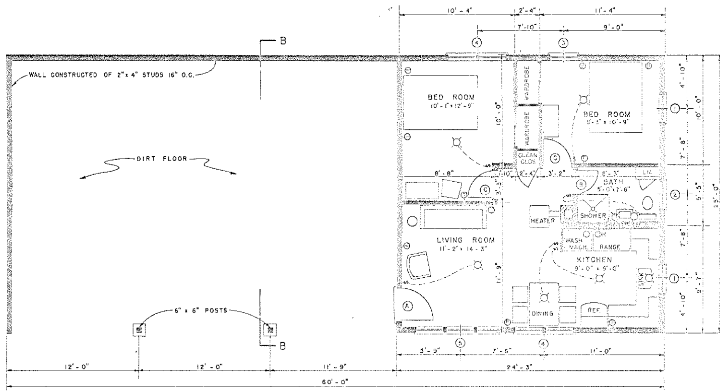
FLOOR PLAN SCALE — 1/2" = 1'-0"
