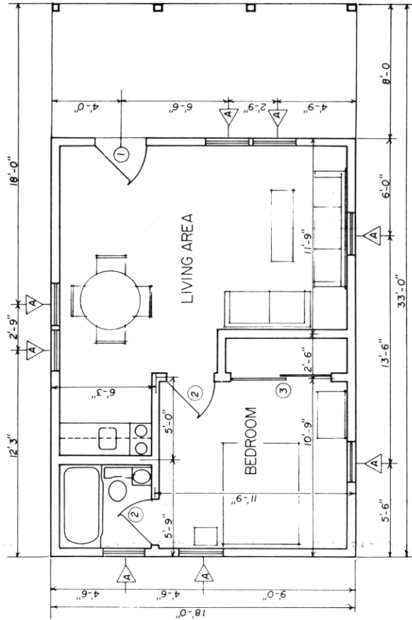
FLOOR PLAN
