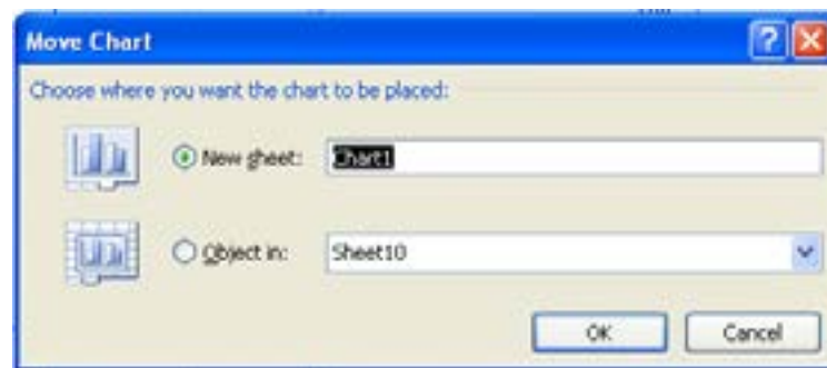
Figure 106: Move Chart.
