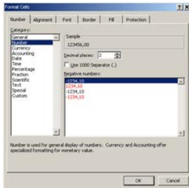
Figure 36: Formatting numbers.
