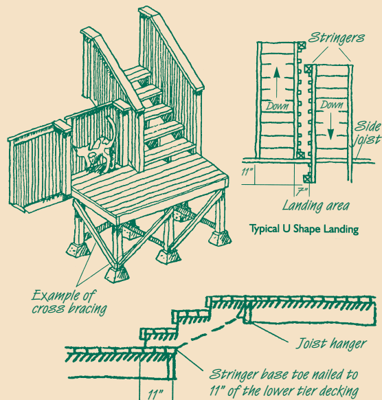
Connecting Stairs Between Tiers
