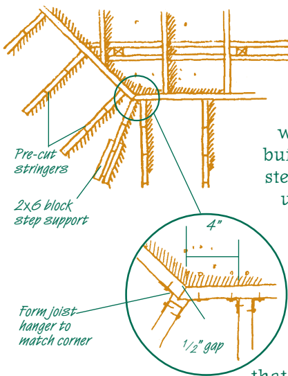
Wraparound Stair Detail
