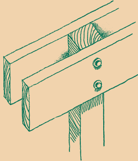
Post to 2x Beam Connection
