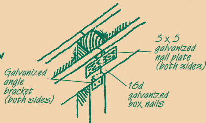
Double Beam Spliced Connection
