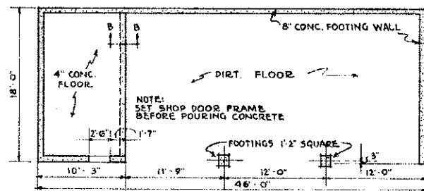
FOOTING PLAN SCALE \frac{1}{8}'' = 1'-0''
