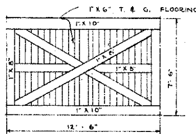
DETAIL OF DOORS SCALE \frac{1}{4}'' = 1'-0''
