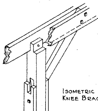
DETAIL OF BRACING SCALE \frac{1}{8}'' = 1'-0''
