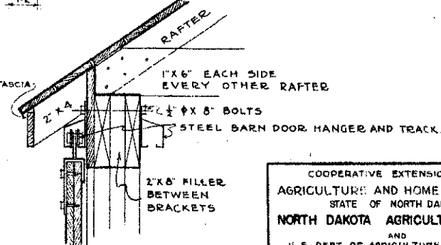
DETAIL OF LINTEL OVER ROLLING DOORS SCALE \frac{1}{4}'' = 1'-0''
