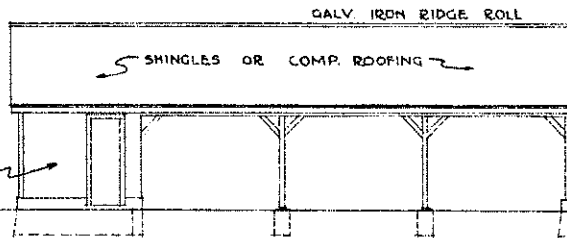
FRONT ELEVATION SCALE \frac{1}{8}'' = 1'-0''
