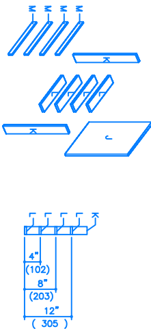
SHELF DETAIL FIGURE 6
