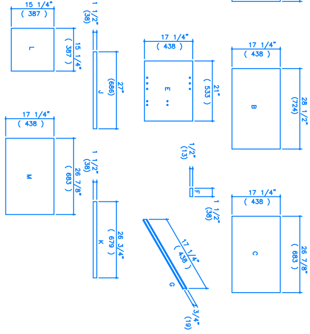
CUTTING DIAGRAM FIGURE 2
