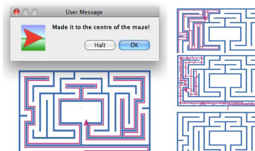
Figure 5.9: How the different turtle behaviours in the Mazes model explore the Hampton Court maze – left: Wall Following; top right: Random Forward 0; middle right: Random Forward 1; bottom right: Random Forward 2.
