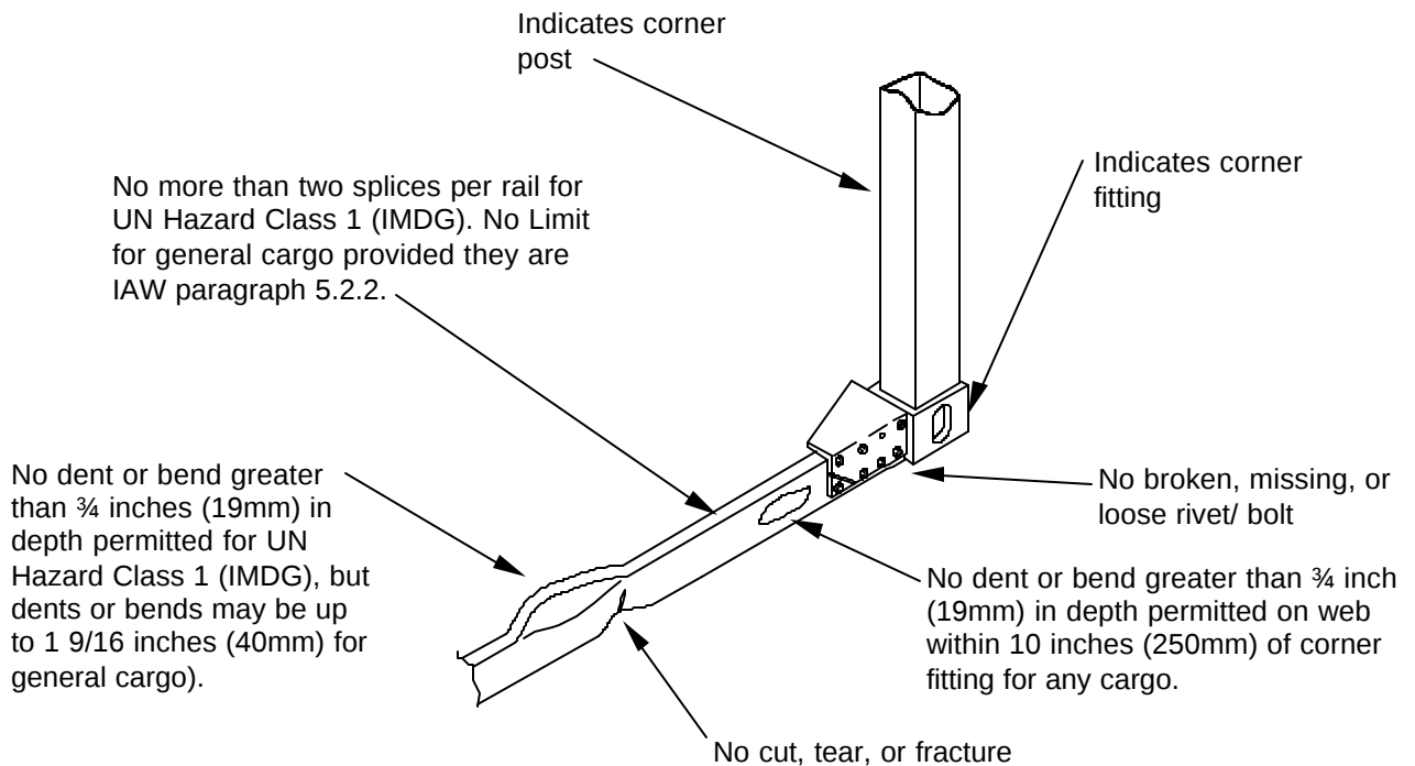
FIGURE 5.2.9B – ALUMINUM SIDE RAIL
