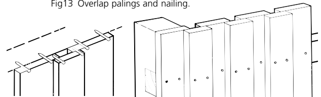
Fig13 Overlap palings and nailing.
