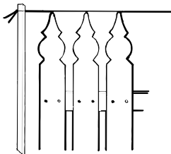
Fig15. Use a spirit level to ensure that picket is vertical. Use a string line to mark the height of the fence.
