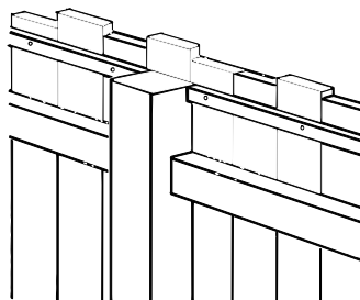
Fig17. Topping the fence.
