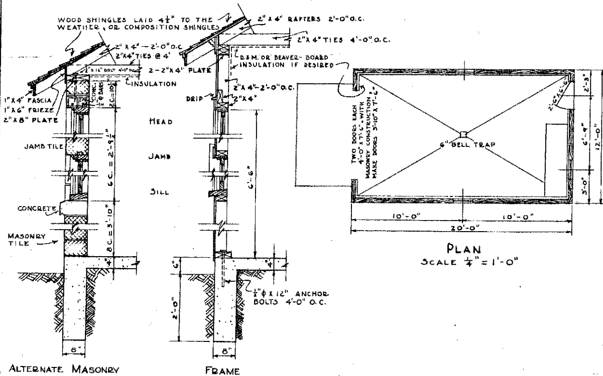
WALL CONSTRUCTIONS SCALE \frac{3}{4}'' = 1'-0''
