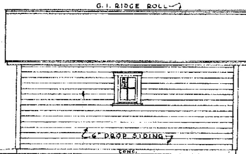
SIDE ELEVATION SCALE \frac{1}{4}'' = 1'-0''
