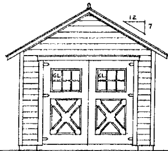
FRONT ELEVATION SCALE \frac{1}{4}'' = 1'-0''
