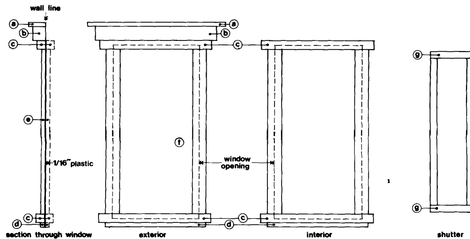
WINDOW DETAILS
