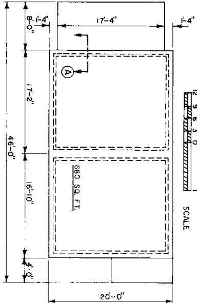
FOUNDATION PLAN
