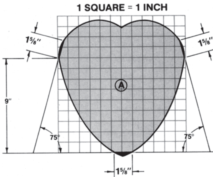
FIGURE 2 SHELF DESIGN
