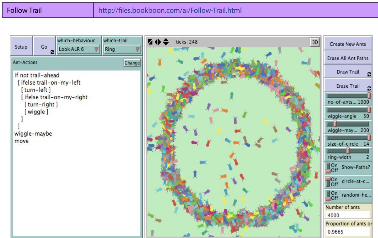
Figure S-5.5.2.1. Screenshot of the Interface for the Follow Trail model after the Setup button has been pressed followed by the go button, with the chooser, input box and slider values as shown in the image.
