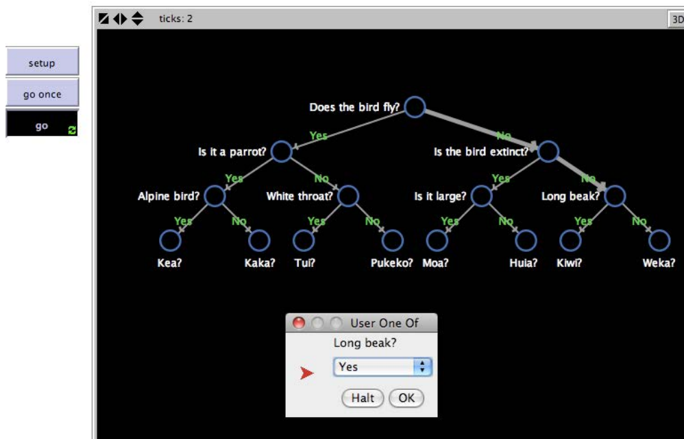
Figure 4.4.4. Screenshot of the Interface for the NZ Birds model after the setup button has been pressed followed by the go button.
