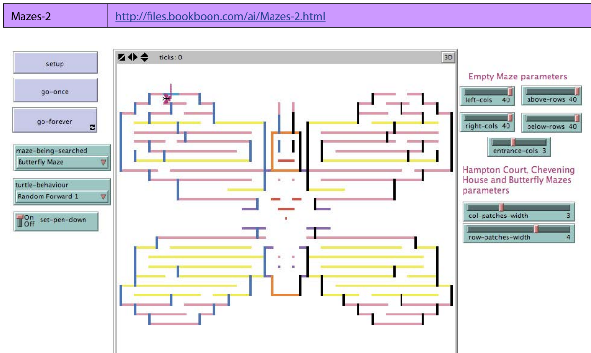
Figure S-5.4.1. Screenshot of the Interface for the Mazes-2 model after the setup button has been pressed followed by the go-forever button, with the chooser and slider values as shown in the image.
