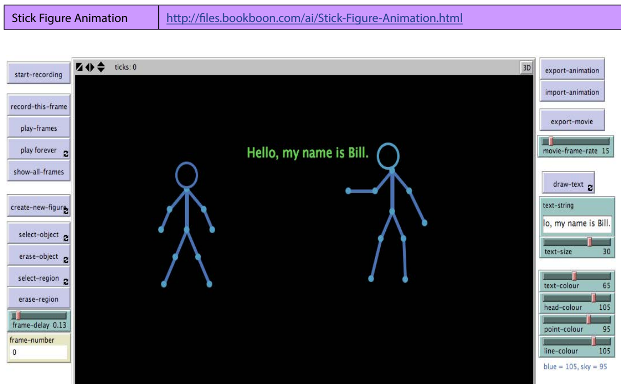
Figure 4.5.3. Screenshot of the Interface for the Stick Figure Animation model after: first, the start-recording button has been pressed; then second, two stick figures have been added to the environment using the create-new-figure button, with the right one altered using the select-object and select-region buttons; and then third, some text added using the draw-text button.
