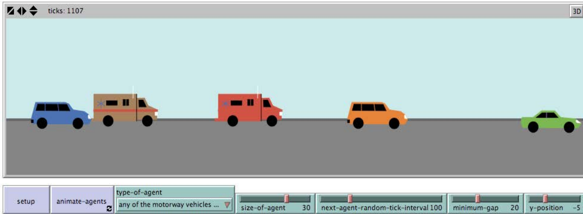
Figure S-4.5.5. Screenshot of the Interface for the Agent Animation model after the setup button has been pressed followed by the animate-agents button, with the slider values as shown in the image.
