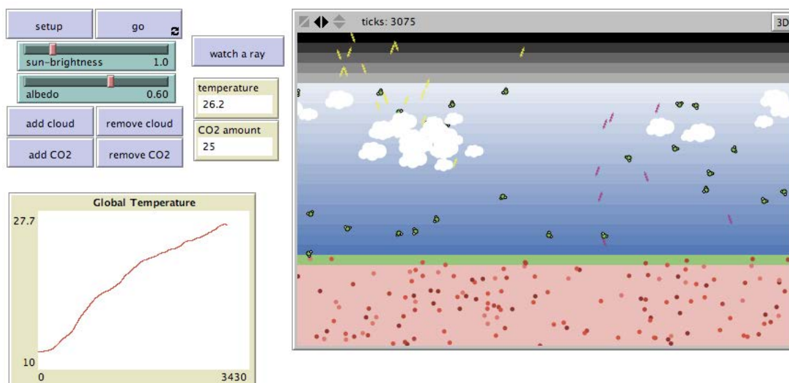
Figure 3.5.4. Screenshot of the Interface for the Climate Change model after the setup and go buttons have been pressed with some clouds and CO 2 added subsequently using the add cloud and add CO2 buttons.
