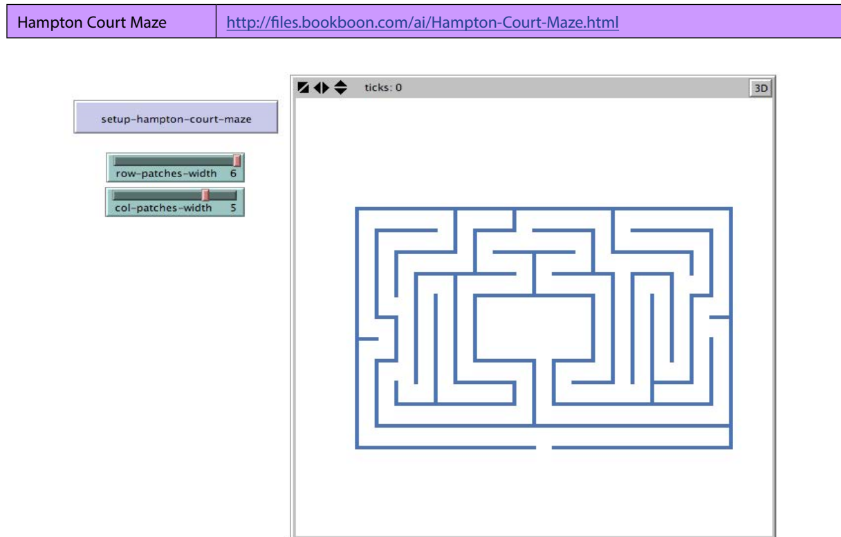
Figure 3.7.1. Screenshot of the Interface for the Hampton Court Maze model after the setup-hampton-court-maze button has been pressed. The entrance to the maze is in the middle bottom, and the goal is to get to the centre of the maze.
