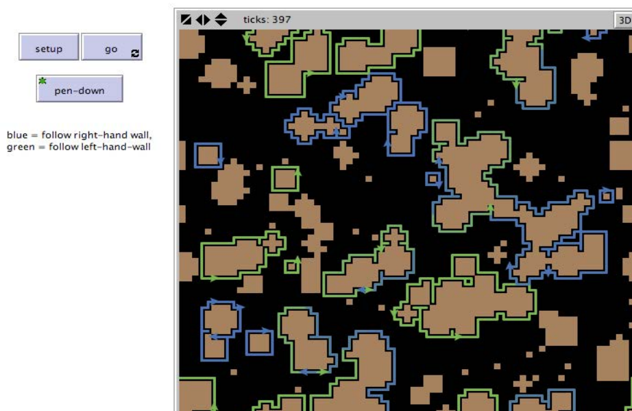
Figure 5.3.1.2 Screenshot of the Interface for the Wall Following model after the setup button has been pressed followed by the pen-down and go buttons.
