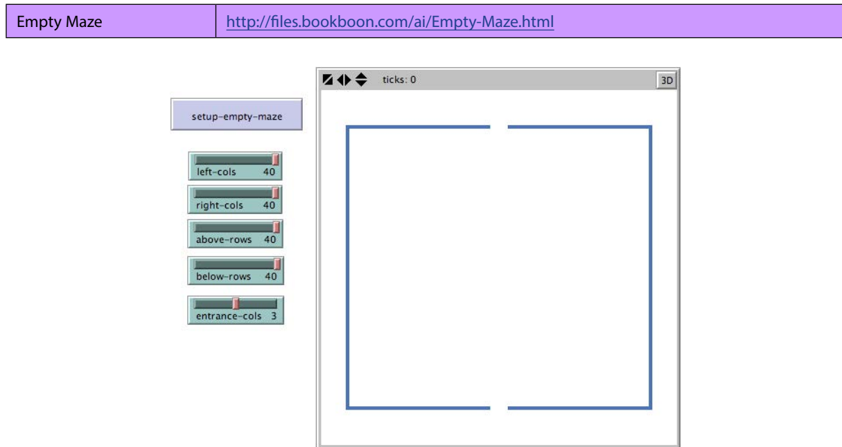
Figure 3.6.7. Screenshot of the Interface for the Empty Maze model after the setup-empty-maze button has been pressed. The entrance to the maze is in the middle bottom, and the goal is to get to the other side of the maze.
