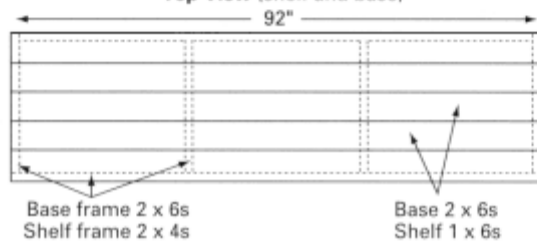
Top View (shelf and base)
