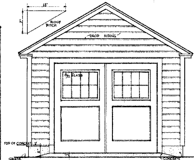
FRONT ELEVATION
