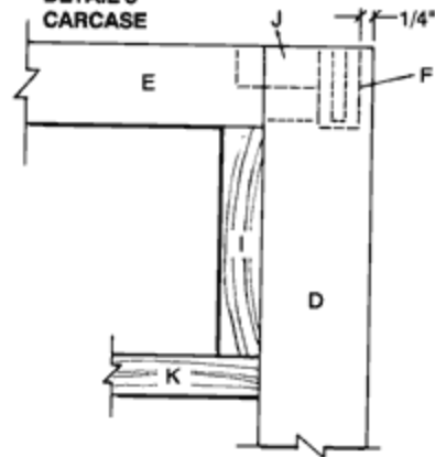
DETAIL 3 CARCASE
