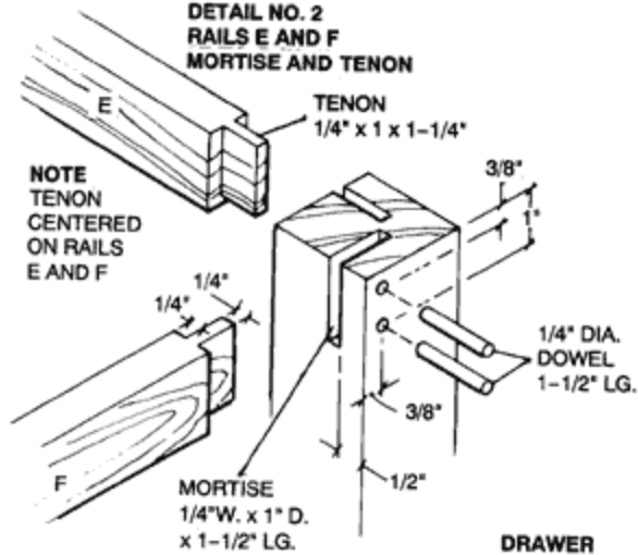
DRAWER DETAIL
