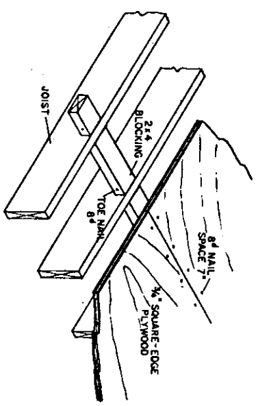
BLOCKING BETWEEN JOISTS FOR SQUARE-EDGE PLYWOOD (NO SCALE)
